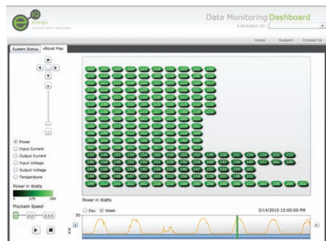
eIQ Parallax vBoost units raise voltage and are wired in parallel to capture maximum power. Because these units can accept up to 350 W, more than one module can be wired to each unit.
